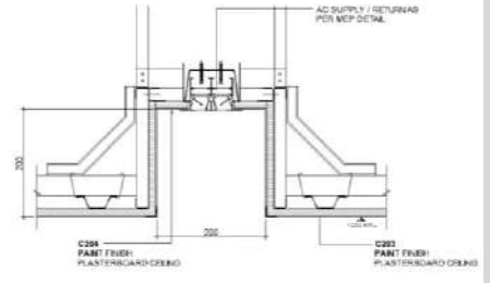
CEILING LINEAR A/C SECTION DETAIL SCALE 1:5
